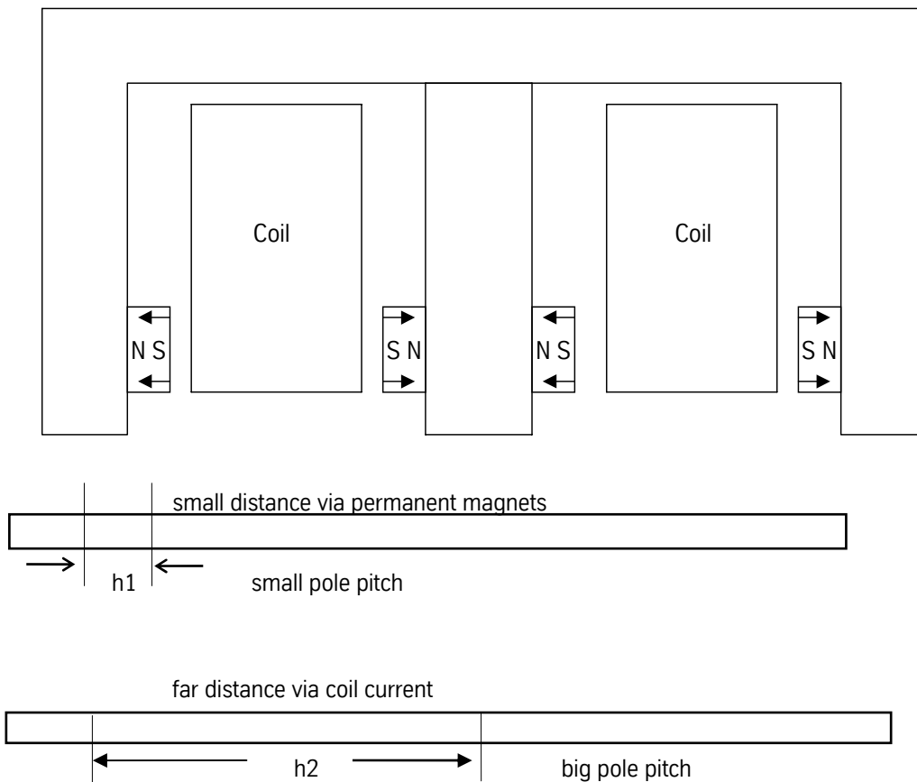
Fig. 6: Representation of the two pole pitches in one system
