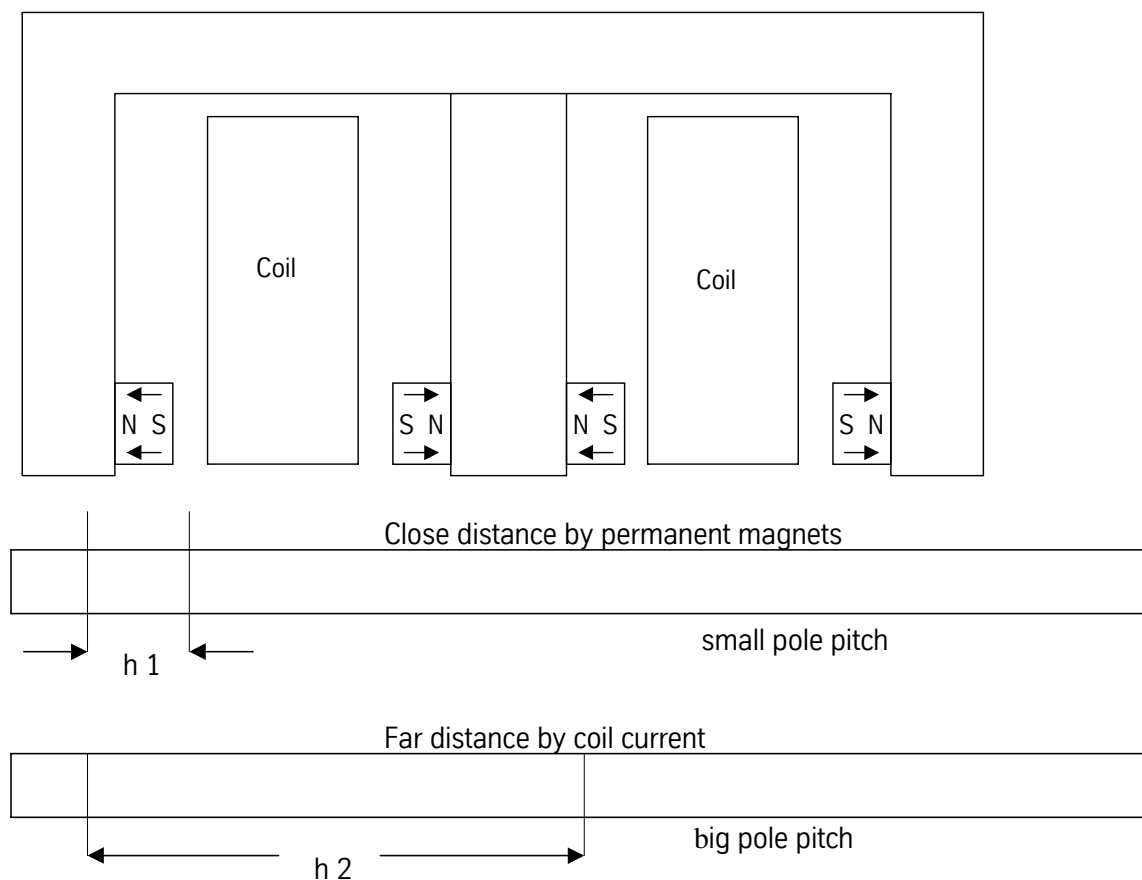
Fig. 3: Representation of the two pole pitches in one system
