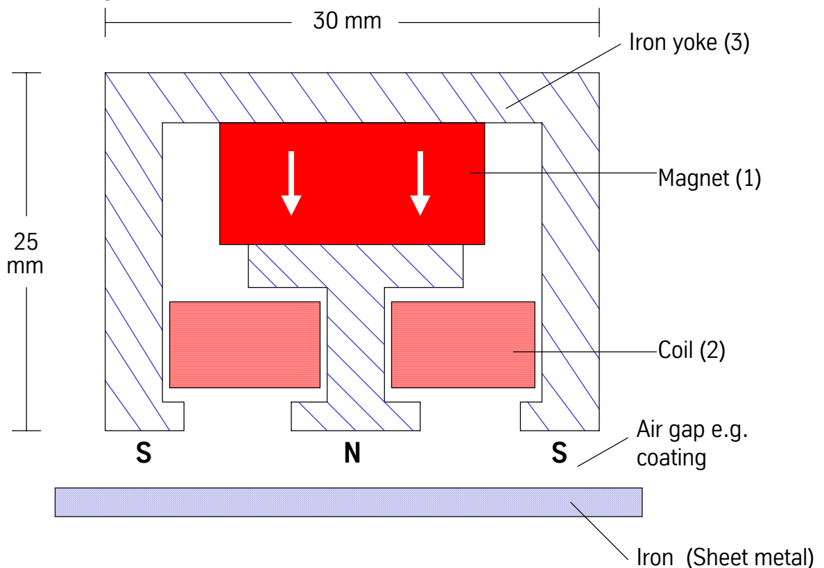
Fig. 2: Monostable displacement system with 1 - magnet, 2 coil and 3 - iron items
