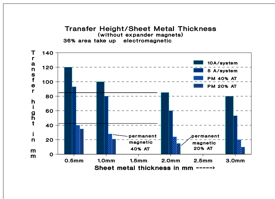
Fig. 4: Transfer heights of the electromagnetic system part in comparison with the permanent magnetic system part
